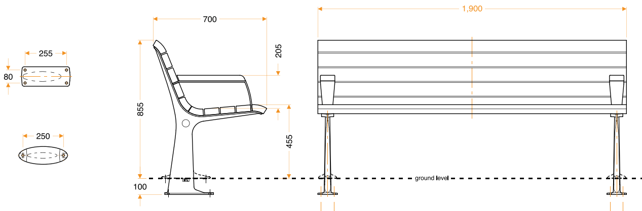
HC2025S Seat (with arms rests)
