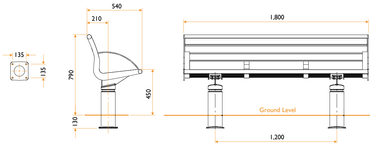
➤ HC2045S Seat with extra dividing arms
